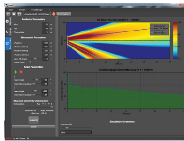
2 Beams @ +5° | -20°
