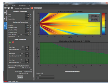
3 Beams @ +20° | -2° | -20°
