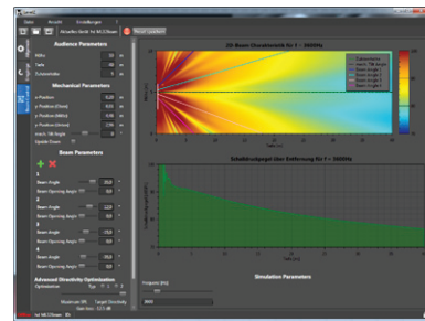
4 Beams @ 35° | +12° | -12° | -35°
