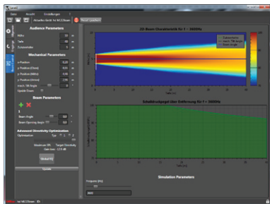
Haupt-Beam @ 0^\circ
