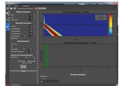
Haupt-Beam @ -32^\circ
